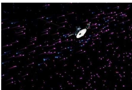
Voyager 1 is now in a new region of the heliosheath, a magnetic highway that is allowing low-energy particles out of the heliosphere and high-energy cosmic rays in.
