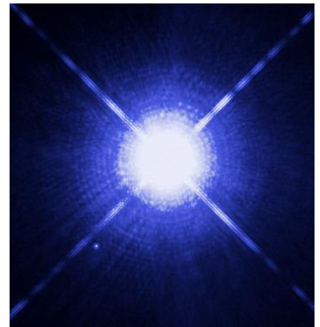
The Dog Star Sirius, which is the brightest star in the sky, is a double star with a white dwarf partner (nicknamed 'the Pup') both located 8.6 light years from the Sun. However no planets have yet been found in the Sirius system. Image: NASA/ESA/H Bond (STScI)/M Barstow (University of Leicester).
